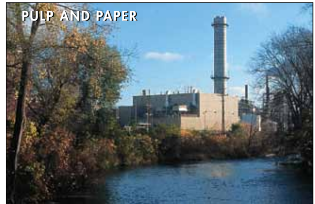
Two 10.7 MW Mars 100 generator sets with SoLoNOx low emissions technology provide cogeneration at this pulp and paper mill in Otsego, Michigan, U.S.A.
